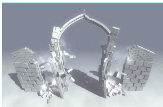
Simulation of a medieval church section failing under seismic loading
